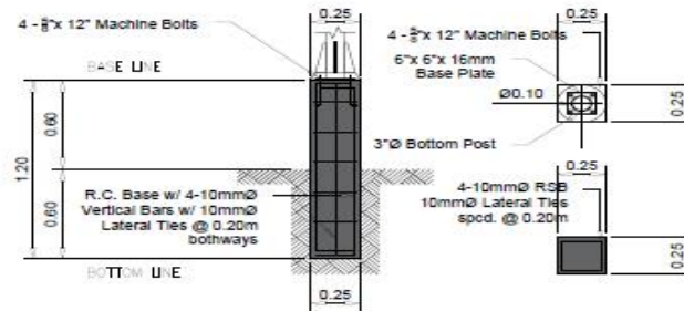
DETAIL OF BASE
