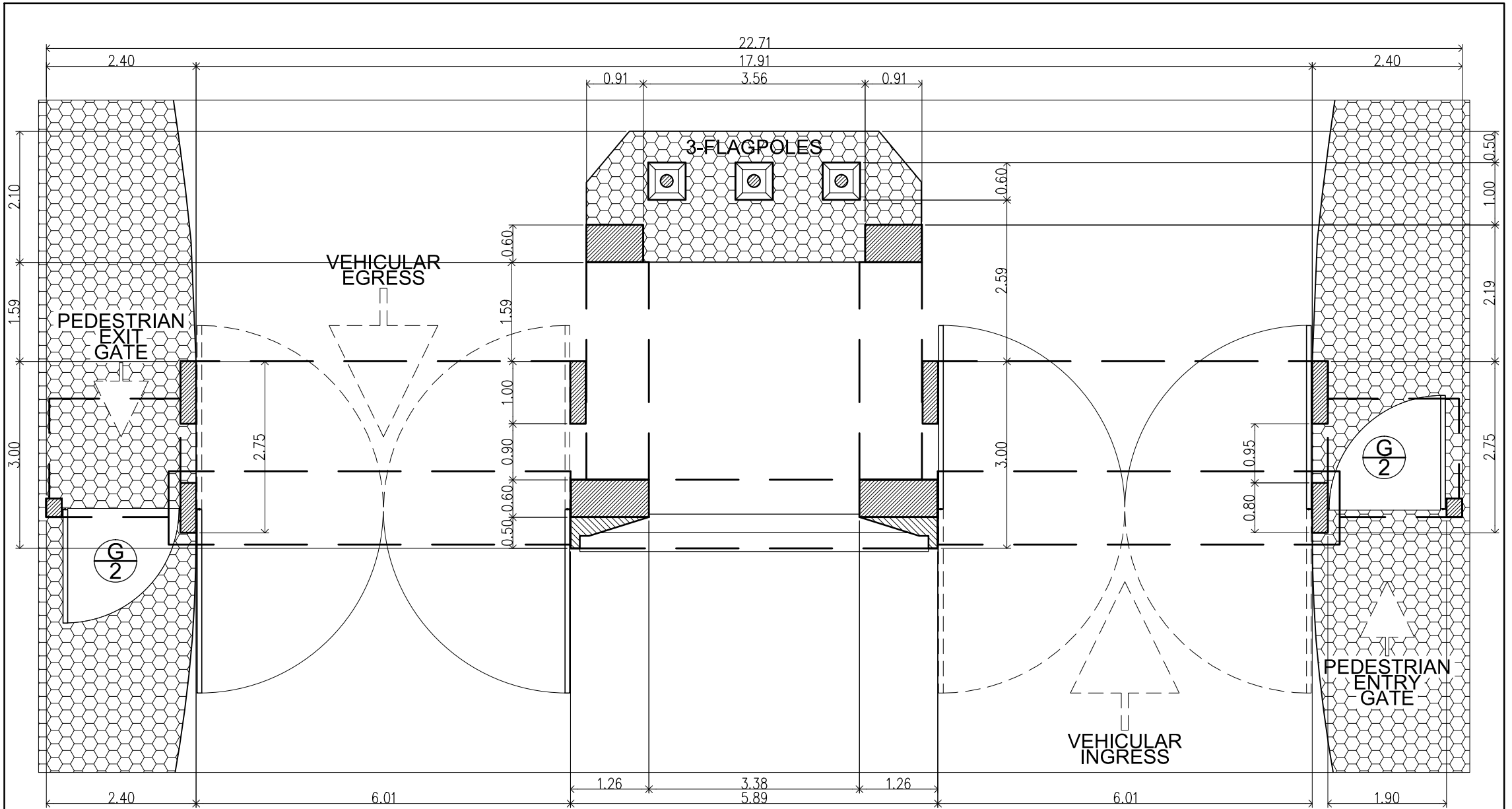
MAIN GATE LAYOUT SCALE: 1/8M
