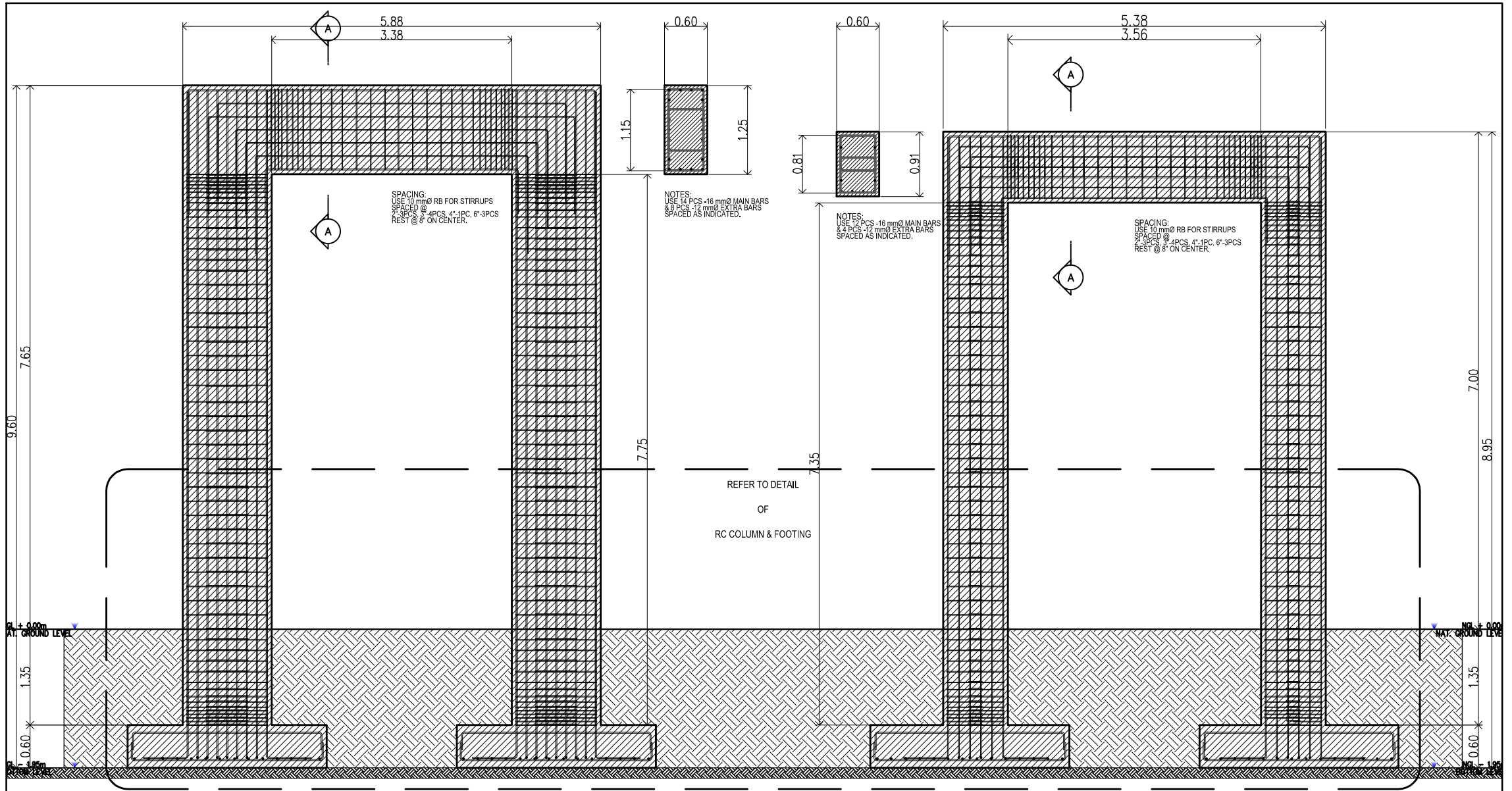
STRUCTURAL DETAIL OF ARCH-1
